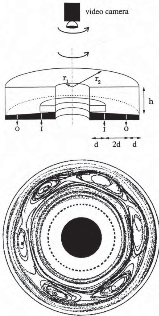
Fig. 5.16. Setup of an experiment with coexisting jets and vortices. Upper panel: the rotating annulus. I and O label two rings of holes for pumping and extracting fluid in the sense of the arrows. As explained in the text, under such conditions both jets and vortices form in the tank. Lower panel: streaks formed by 90-second-long trajectories of about 30 tracer particles reveal the presence of six vortices sandwiched between two azimuthal jets. The picture has been taken in a reference frame corotating with the vortex chain. By courtesy of H. Swinney. Reprinted with permission from Elsevier Science from T. H. Solomon et al.: Physica D 76 , 70 (1994). ©1994 Elsevier Science
